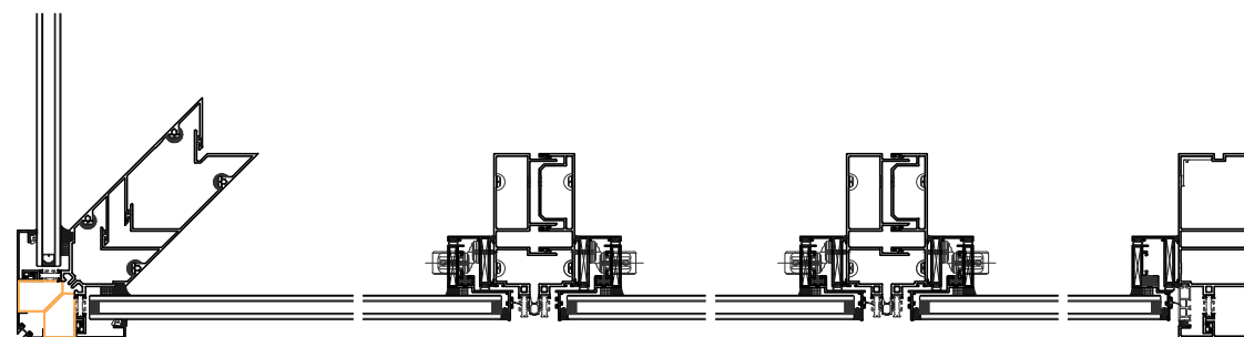
2 HORIZONTAL SECTION DETAIL
